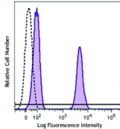
HeLa cells (open histogram) and HeLa cells treated with Nocodazole for 24 hours (filled histogram), were fixed, permeabilized, and then stained with anti-Histone H3-Phosphorylated (Ser28) (clone HTA28) PerCP/Cy5.5.
