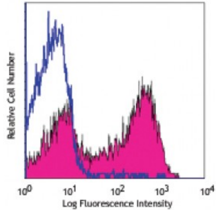
C57BL/6 splenocytes stained with 11-26c.2a PerCP/Cy5.5
