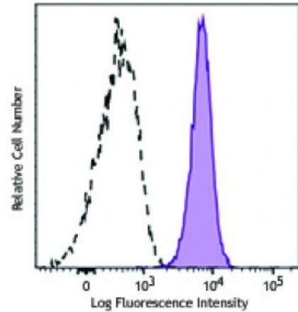
Cell line U937 was stained with human MERTK (clone 590H11G1E3) PE/Cy7 (filled histogram) or mouse IgG1, \kappa PE/Cy7 isotype control (open histogram).
