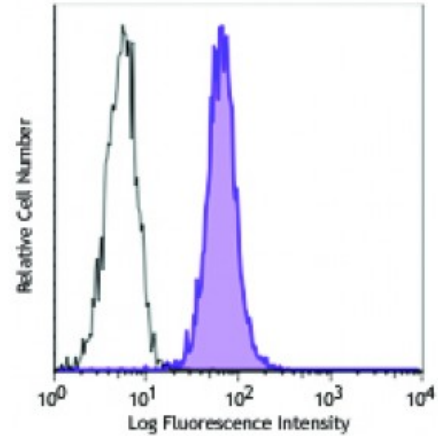
Human teratocarcinoma cell line NCCIT was stained with ROR1 (clone 2A2) PE/Cy7 (filled histogram) or mouse IgG1, κ PE/Cy7 isotype control (open histogram).
