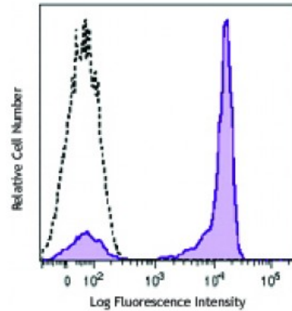
Human peripheral blood lymphocytes were stained with CD27 (clone M-T271) PE (filled histogram) or mouse IgG1 PE isotype control (open histogram).
