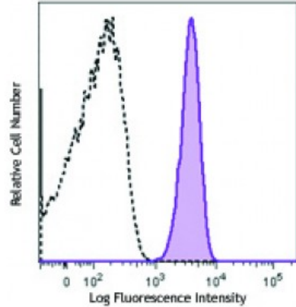
Human red blood cells were stained with anti-human CD235a (clone HI264) PerCP/Cy5.5 (filled histogram) or mouse IgG2a, κ PerCP/Cy5.5 isotype control (open histogram).
