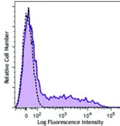
Human peripheral blood lymphocytes were stained with HLA-DR (clone LN3) PE/Cy7 (filled histogram) or mouse IgG2b, \kappa PE/Cy7 isotype control (open histogram).
