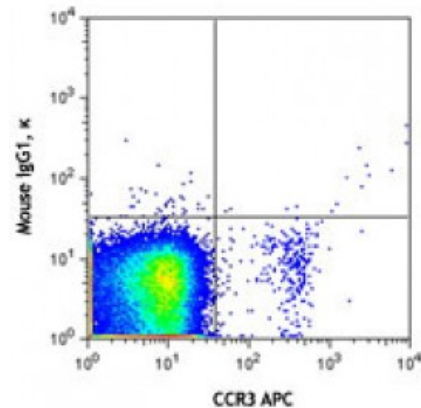
Human peripheral blood leukocytes were stained with CCR3 APC and anti-human IgE (clone MHE-18) PE/Cy7 (top) or mouse IgG1, κ PE/Cy7 (bottom). Data shown was gated on the lymphocyte population.
