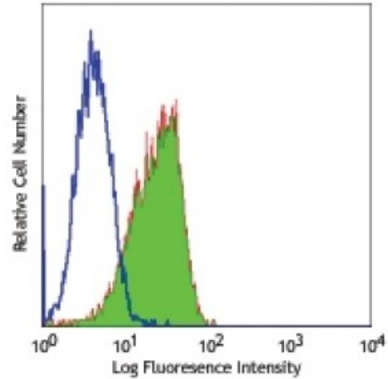
Human colon carcinoma cell line (HT29) stained with purified CD324 (clone 67A4) (filled histogram), or purified mouse IgG1, κ (open histogram) followed by anti-mouse IgG FITC.
