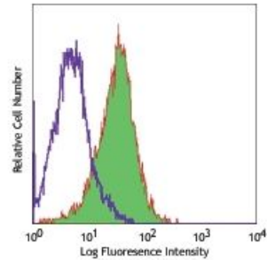
Human pre-B cell line REH stained with BV10A4H2 PE
