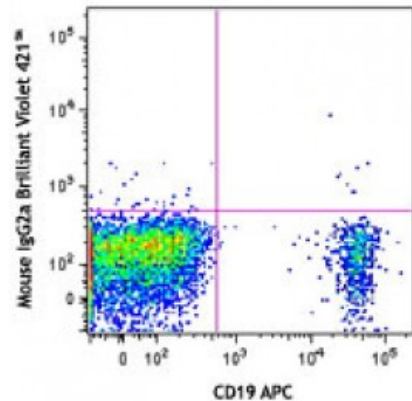
Human peripheral blood lymphocytes stained with CD19 APC and CD24 (clone ML5) Brilliant Violet 421™ (top) or mouse IgG2a, κ Brilliant Violet 421™ isotype control (bottom).
