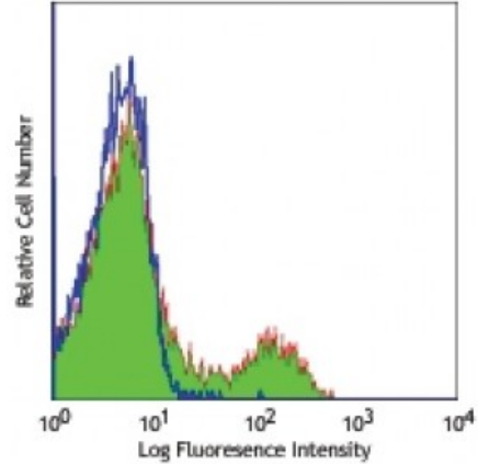
Human peripheral blood lymphocytes stained with purified DX22, followed by anti-mouse IgGs FITC
