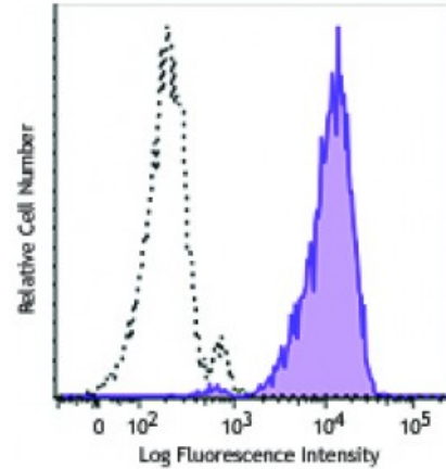
Human peripheral granulocytes were stained with CD13 (clone WM15) PE/Dazzle™ 594 (filled histogram) or mouse IgG1, κ PE/Dazzle™ 594 isotype control (open histogram).
