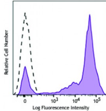
Human peripheral blood lymphocytes were stained with CD5 (clone UCHT2) PE/Dazzle™ 594 (filled histogram) or mouse IgG1, κ PE/Dazzle™ 594 isotype control (open histogram).
