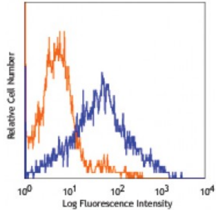
Bone marrow derived-dendritic cells from C57BL/6 mouse stained with purified NLDC-145 conjugated with Alexa Fluor® 647
