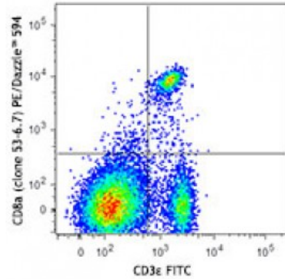
C57BL/6 mouse splenocytes were stained with CD3ε FITC and CD8a (clone 53-6.7) PE/Dazzle™ 594 (top) or rat IgG2a, κ PE/Dazzle™ 594 isotype control (bottom).
