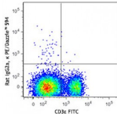
C57BL/6 mouse splenocytes were stained with CD3ε FITC and CD8a (clone 53-6.7) PE/Dazzle™ 594 (top) or rat IgG2a, κ PE/Dazzle™ 594 isotype control (bottom).
