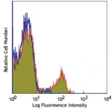
C57BL/6 mouse splenocytes were stained with CD8 (clone 53-6.7) APC/Cy7 (filled histogram) or rat IgG2a, κ APC/Cy7 isotype control (open histogram).
